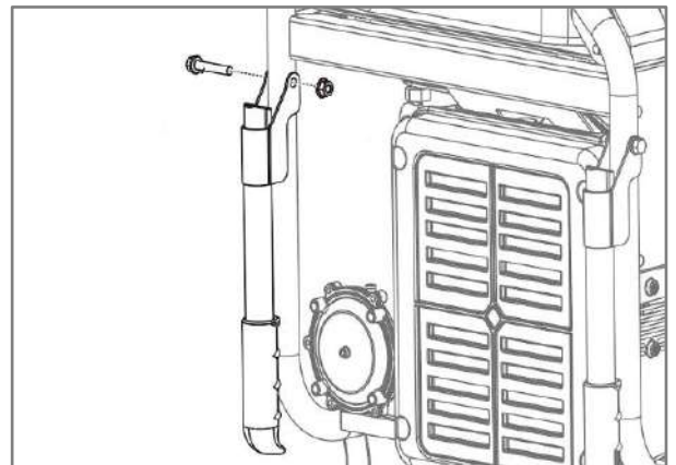
M8 Nut x2 Used for Handle
